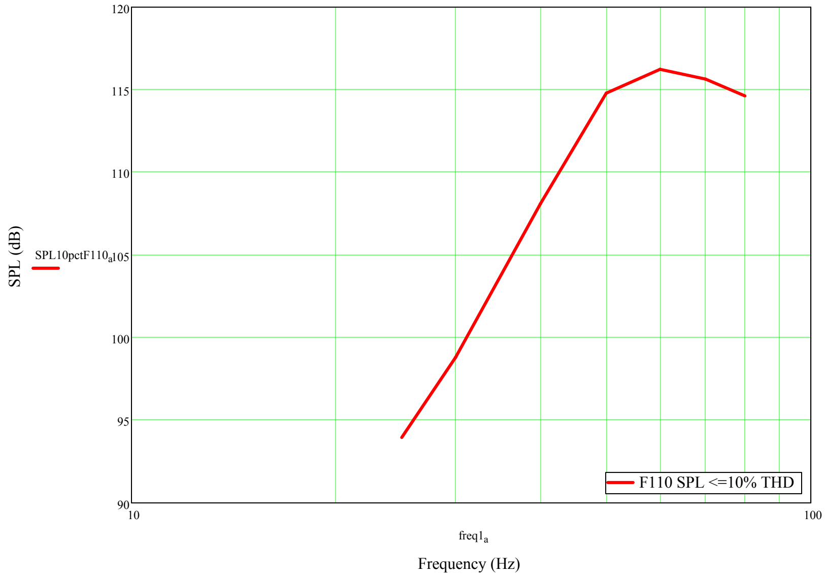
F110, avg SPL at 10% or less THD, 1 meter ground plane, sine stimulus
