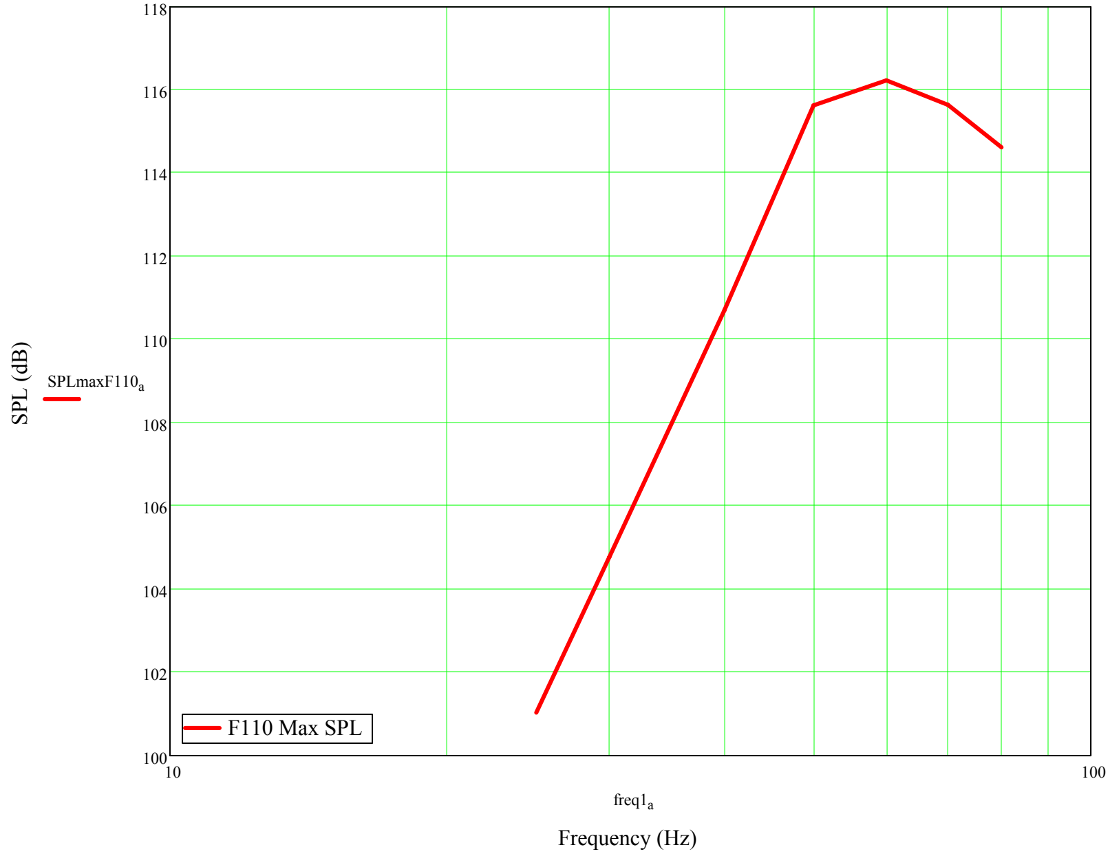
F110, Maximum avg SPL, 1 meter ground plane, sine-wave stimulus
