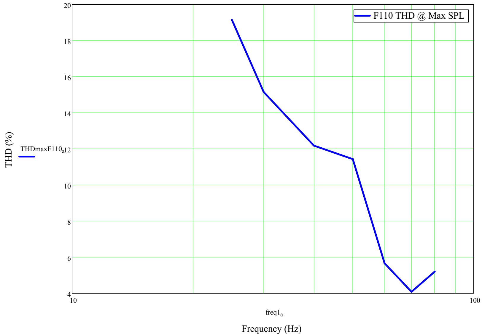
F110, THD at Maximum avg SPL, 1 meter ground plane, sine stimulus
