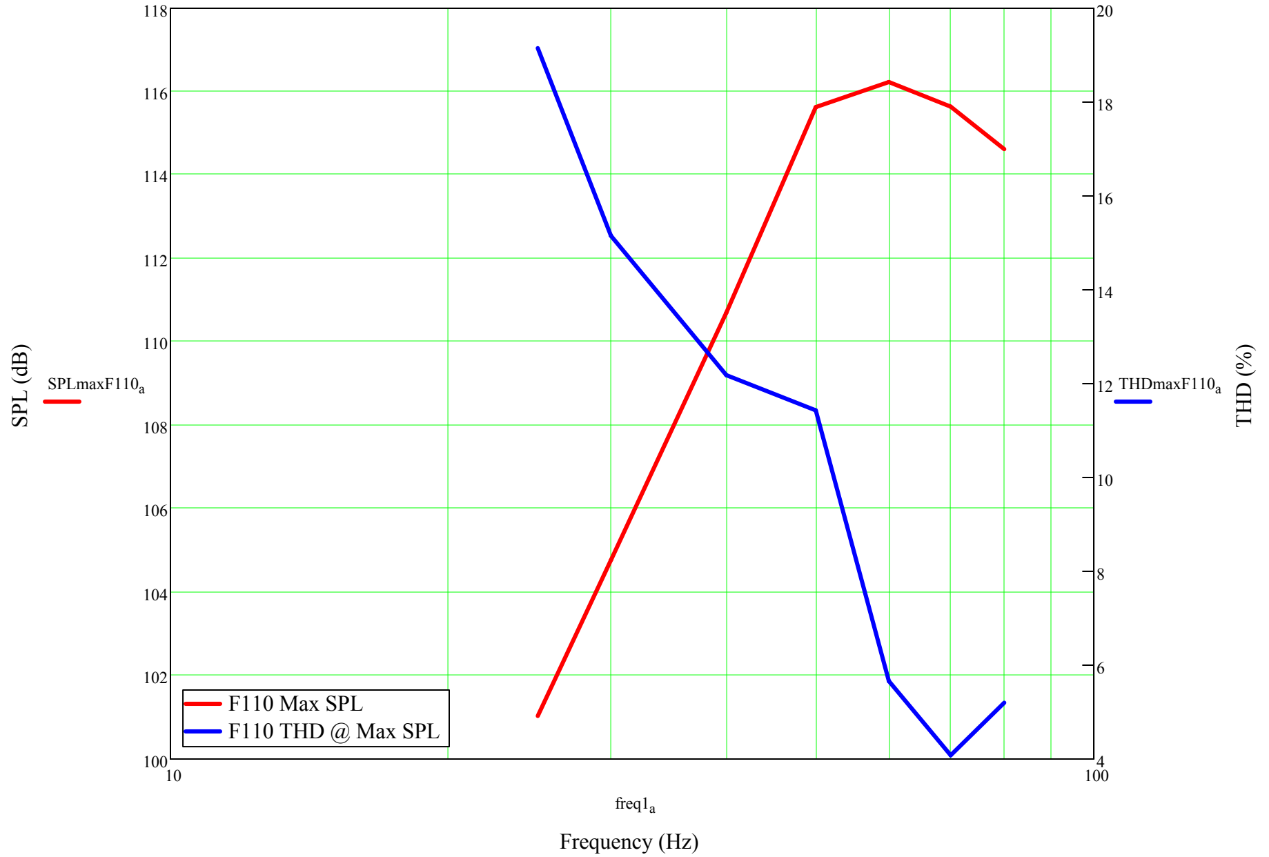
F110, Maximum avg SPL with THD (@ max spl), 1 m ground plane, sine stimulus
